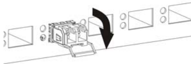
Figure 9 Opening the Transceiver's Latch Example
