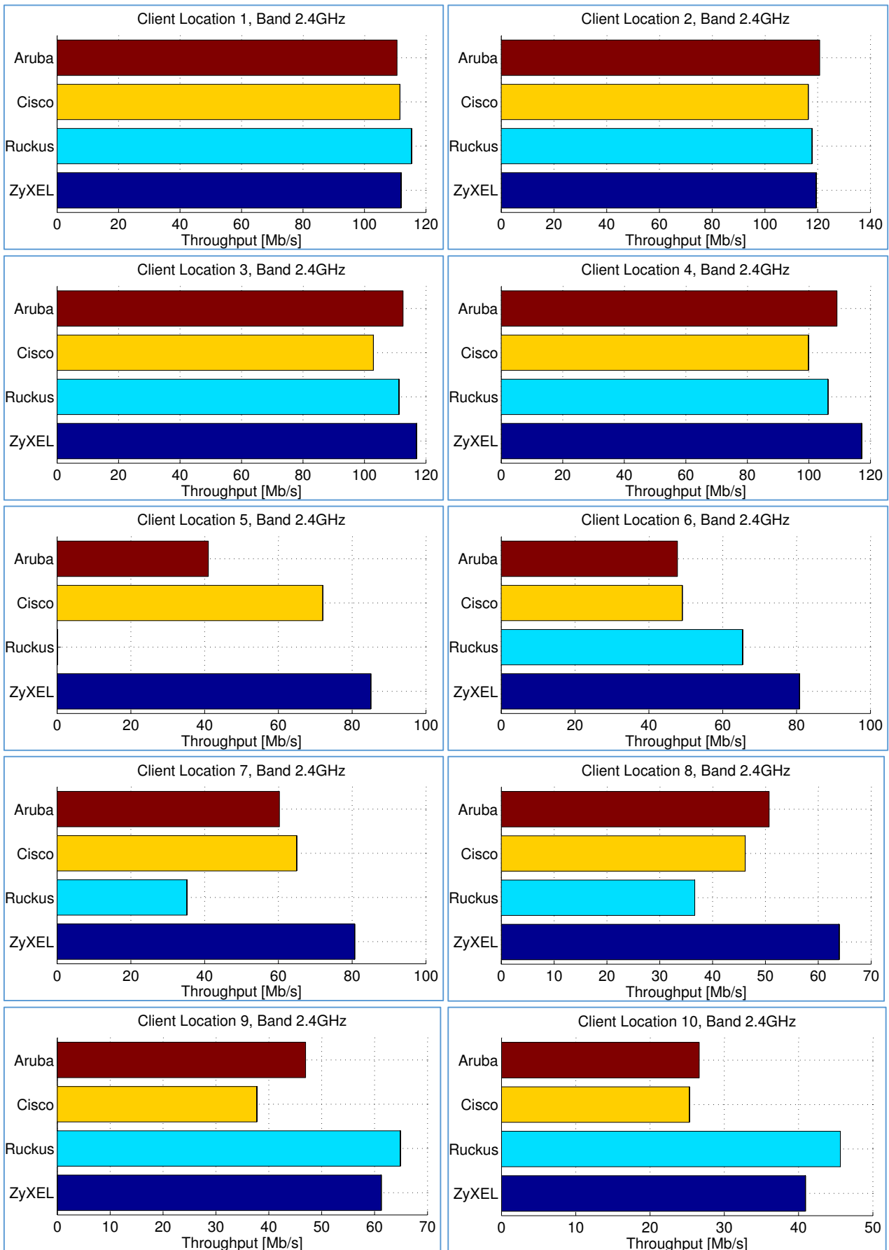
Figure 3 Throughput vs Location difficulty: Band 2.4GHz, downlink
